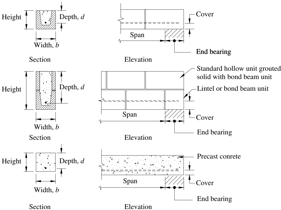
Figure 4-3: Construction Details, Simple Supports
